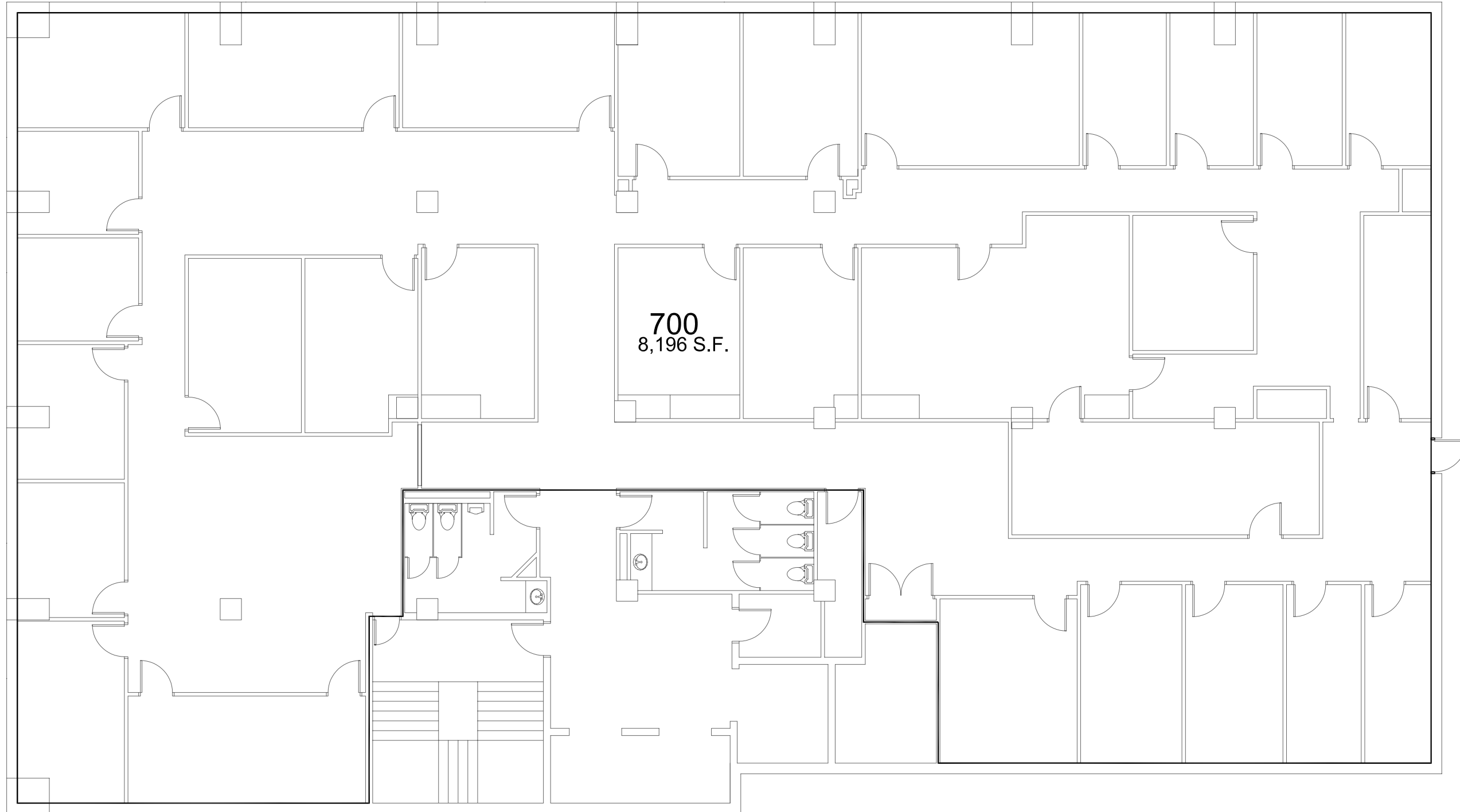
SEVENTH FLOOR PLAN 0 4' 9,562 S.F.
